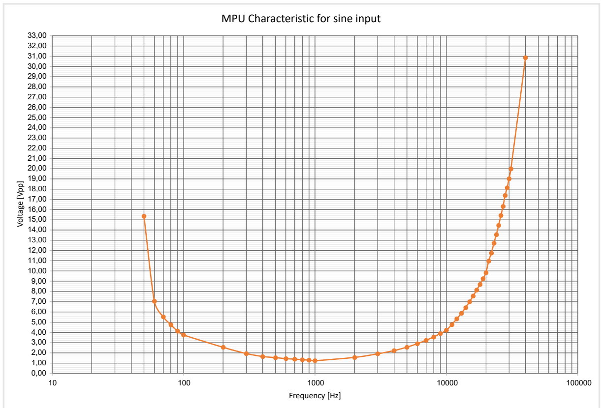
Fig. 64: MPU - characteristic Vpp
