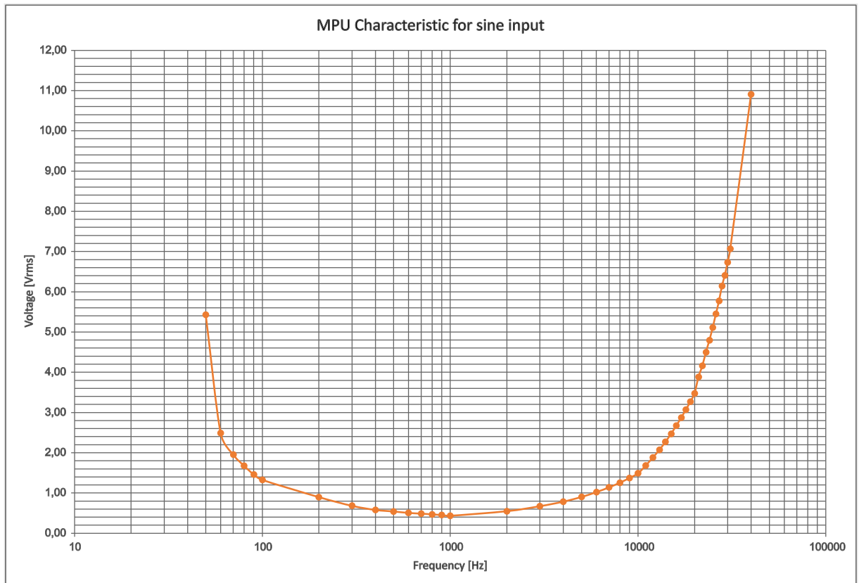
Fig. 63: MPU - characteristic Vrms
